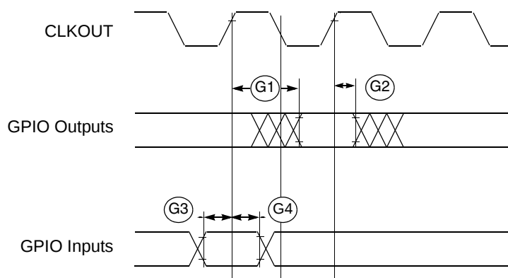
Figure 15. GPIO Timing
